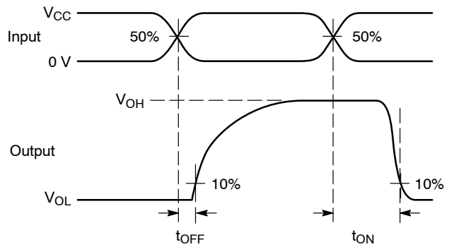
Figure 2. t_{ON}/t_{OFF}
